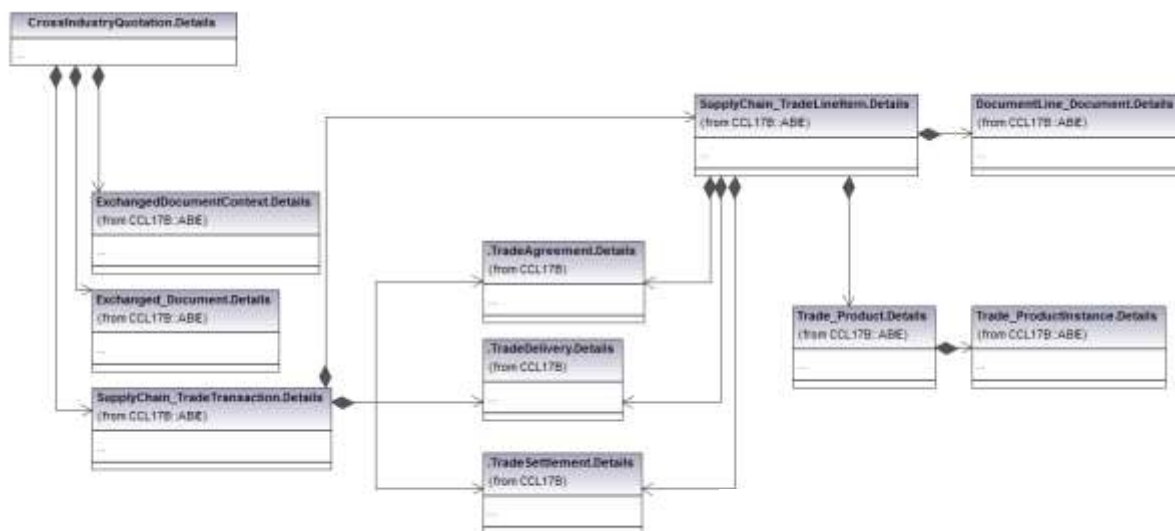
214 Figure 1 Cross Industry Quotation conceptual data model
