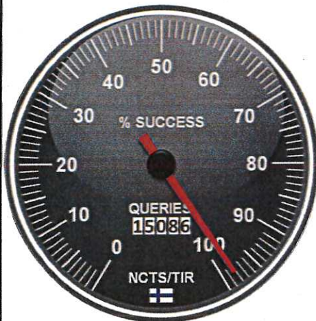
Query graph
