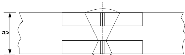
Center of the weld
