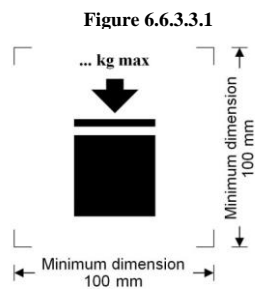
Large packagings capable of being stacked
