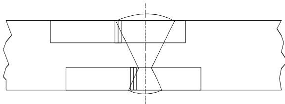
Heat affected zone
