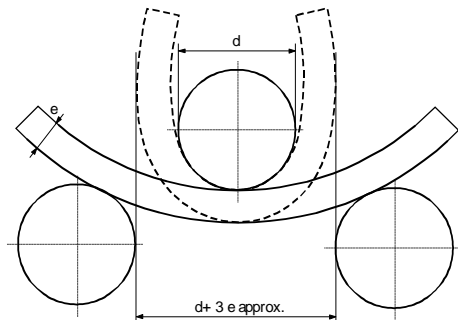
Diagram of bend test
