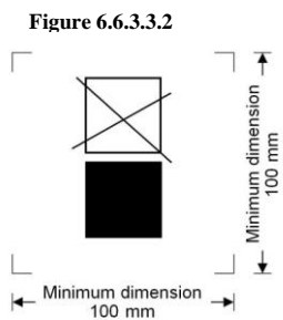
Large packagings NOT capable of being stacked
