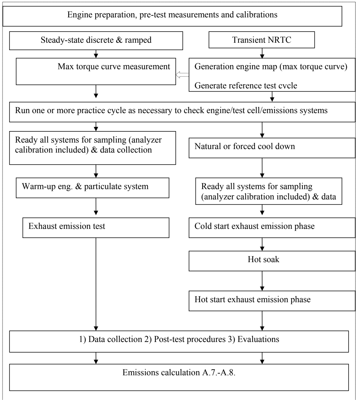
Figure 7.3 – Test sequence
