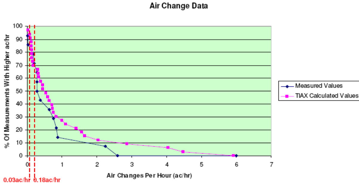
Figure 10: Available Real World Measurements (exc. Canadian studies) & TIAX Calculated Ventilation Rates
