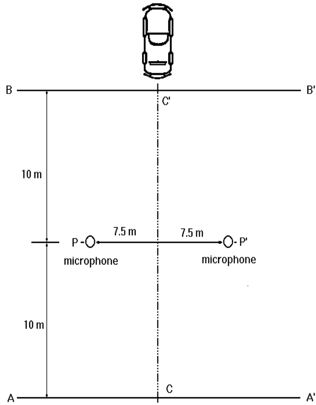
Microphone positions for the measurement
