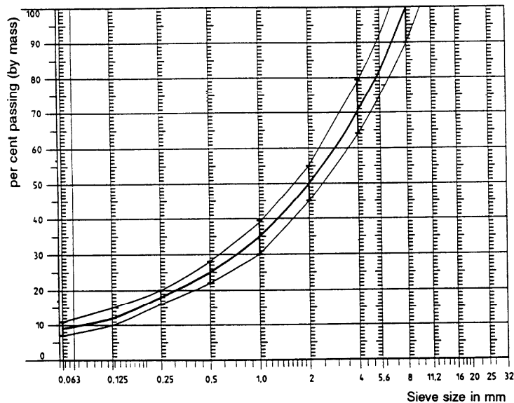
Figure 2 Grading curve of the aggregate in the asphaltic mix with tolerances
