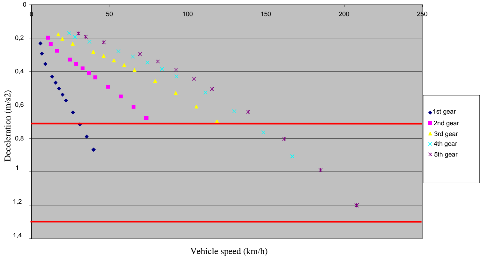
Natural engine brake, M 1 diesel vehicle, 1-5 gear
