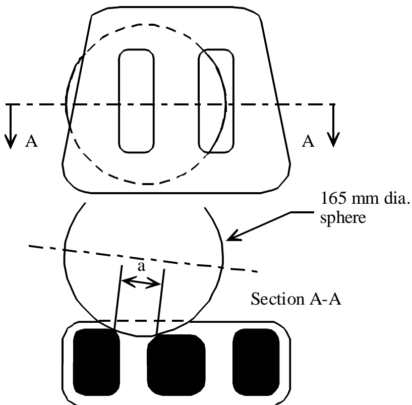
Figure 3-2 Measurement of a horizontal gap "A".
