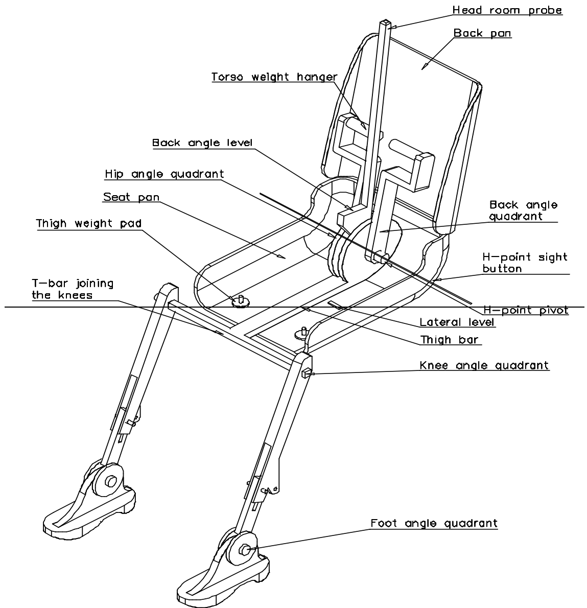
Figure 3-1 3-D H machine elements designation
