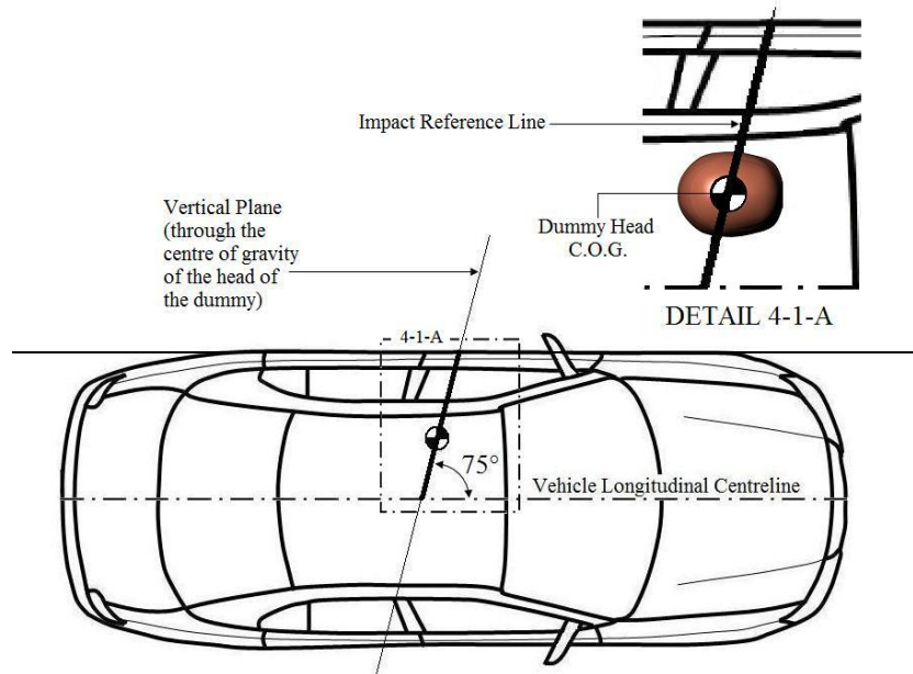
Figure 4-1 Vehicle to be impacted on left side (overhead plan view)
