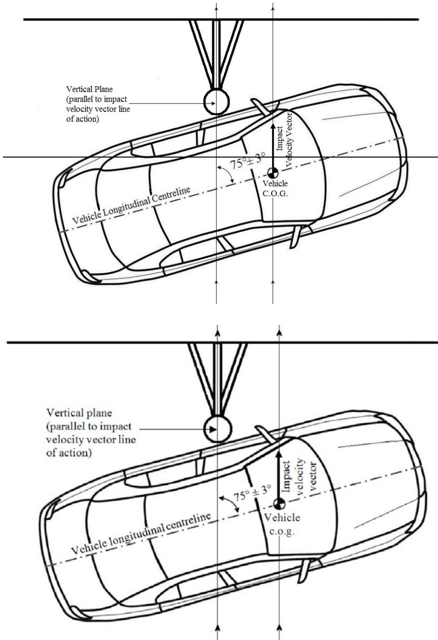
Figure 5-2 Right side impact (overhead plan view)
