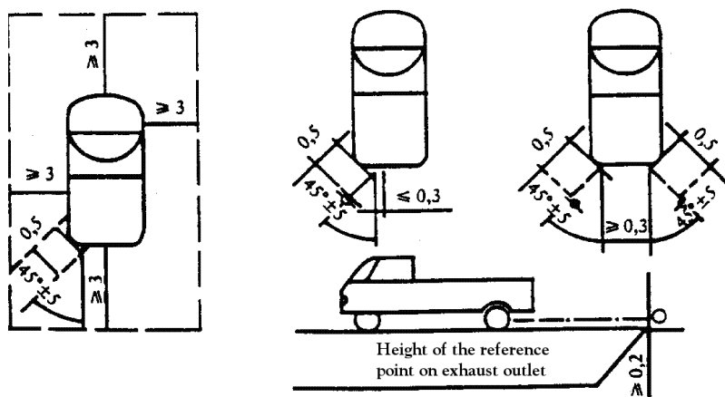
Figure 2 Positions for testing the stationary vehicle
