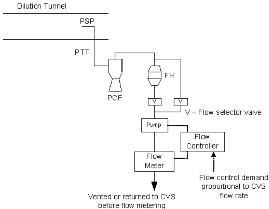
Figure A5/12 Particulate sampling system
