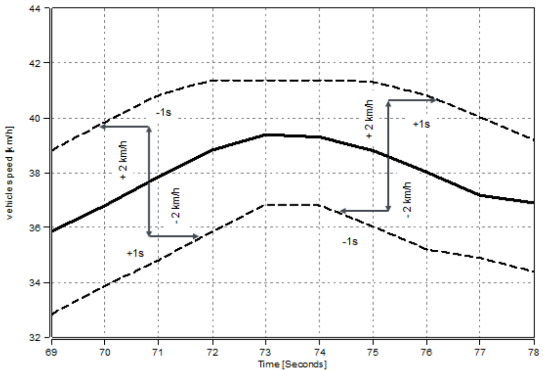
Figure A6/2 Speed trace tolerances
