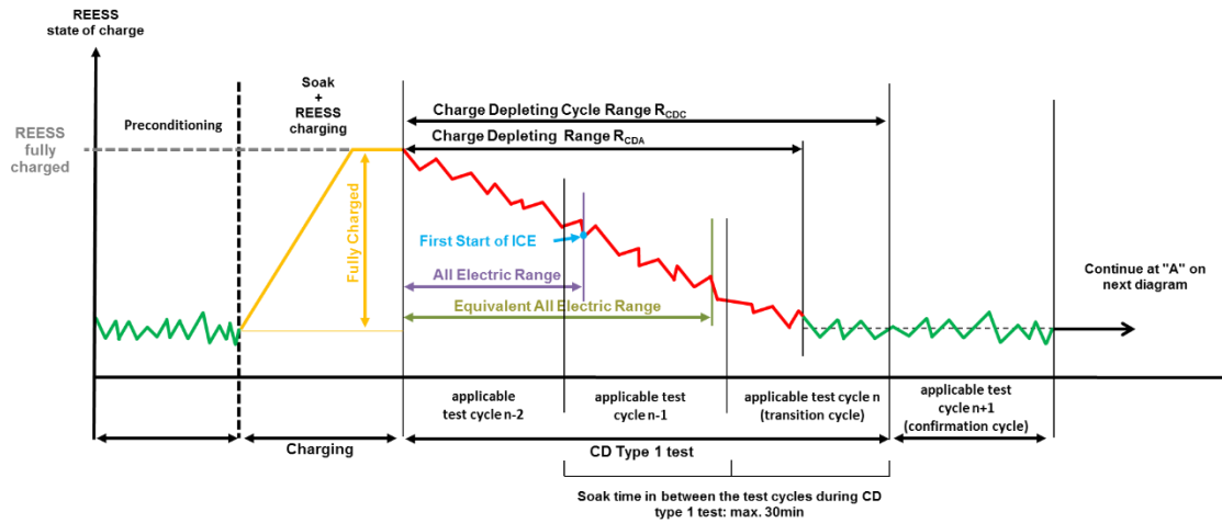
Figure A8.App1/3 OVC-HEVs, charge-depleting type 1 test with subsequent charge-sustaining Type 1 test
