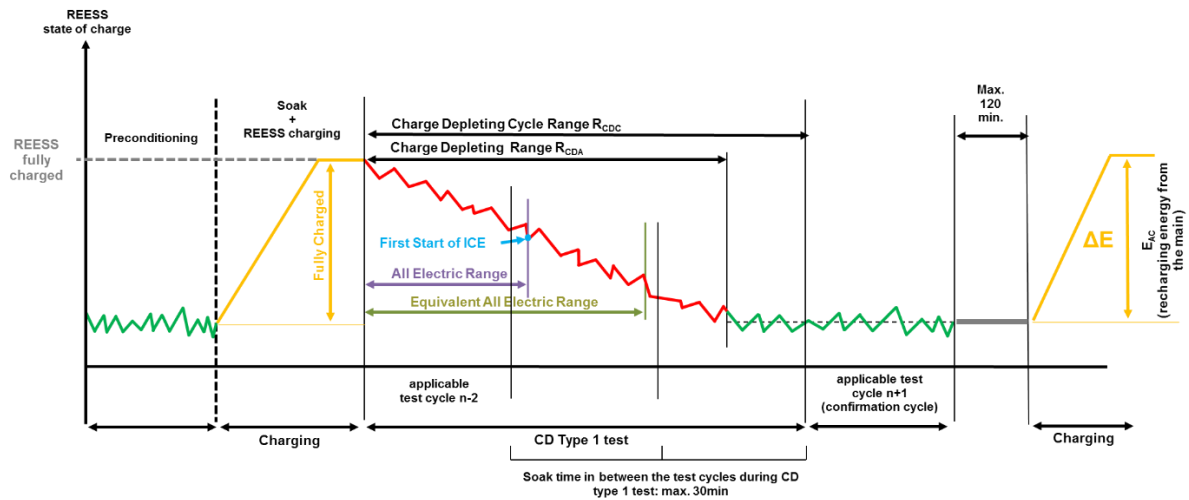
Figure A8.App1/1 OVC-HEVs, charge-depleting Type 1 test
