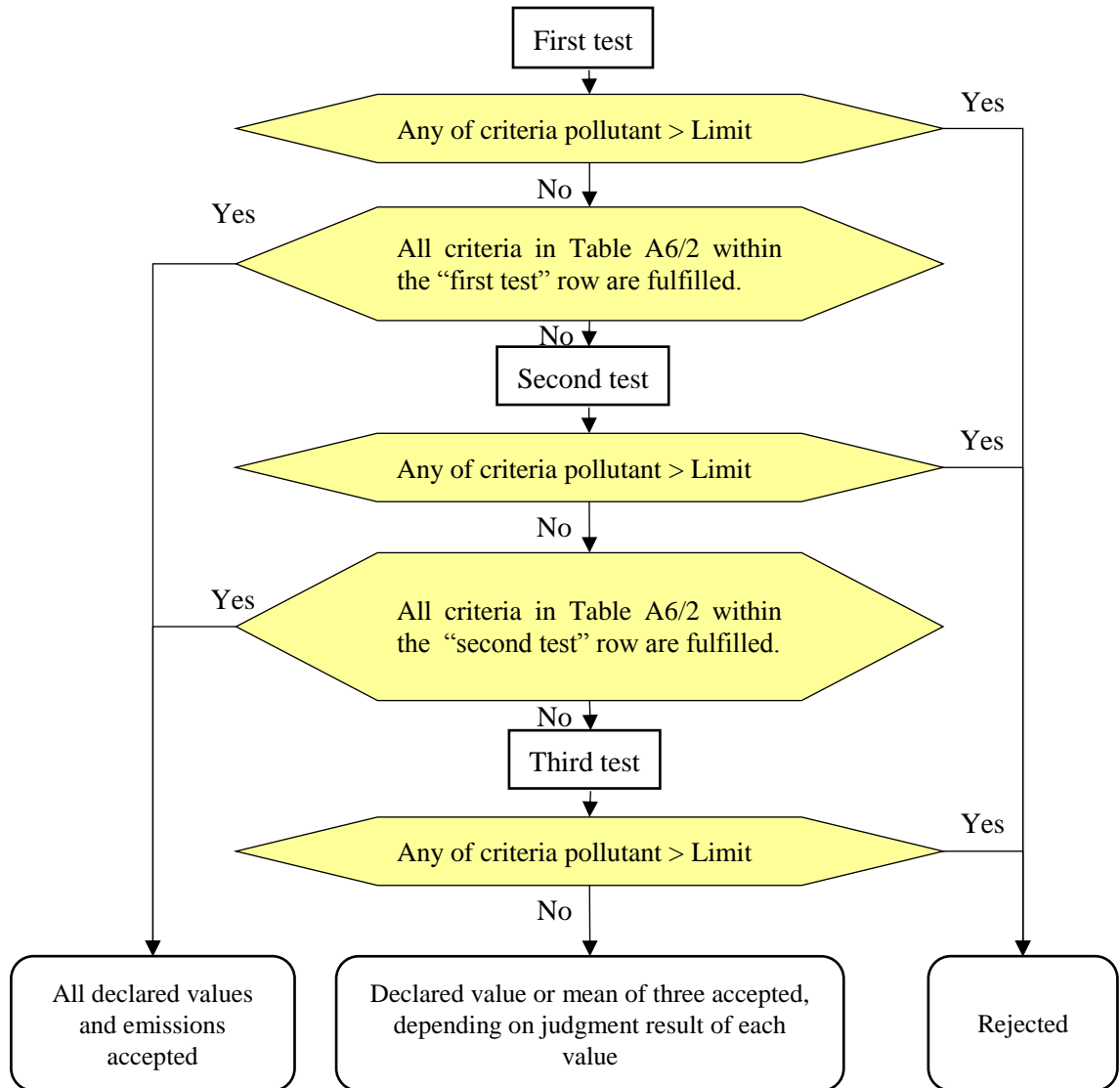
Flowchart for the number of Type 1 tests
