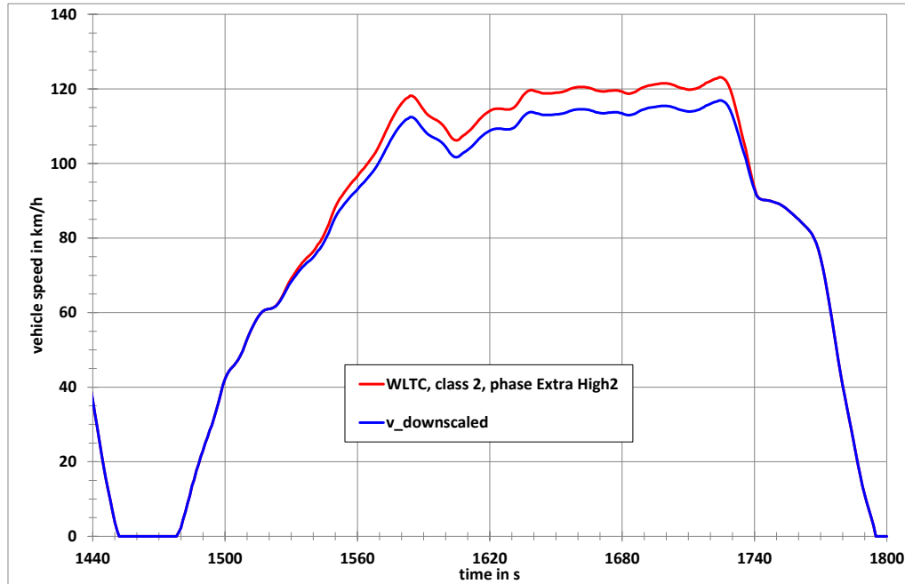
Downscaled extra high speed phase of the Class 2 WLTC
