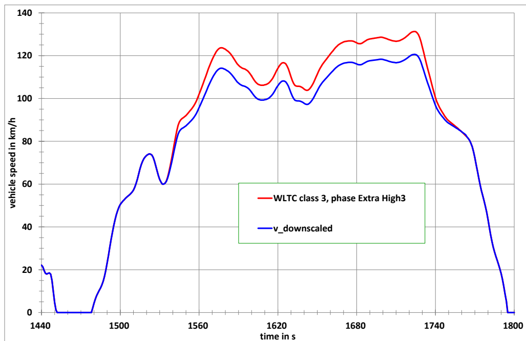
Downscaled extra high speed phase of the Class 3 WLTC
