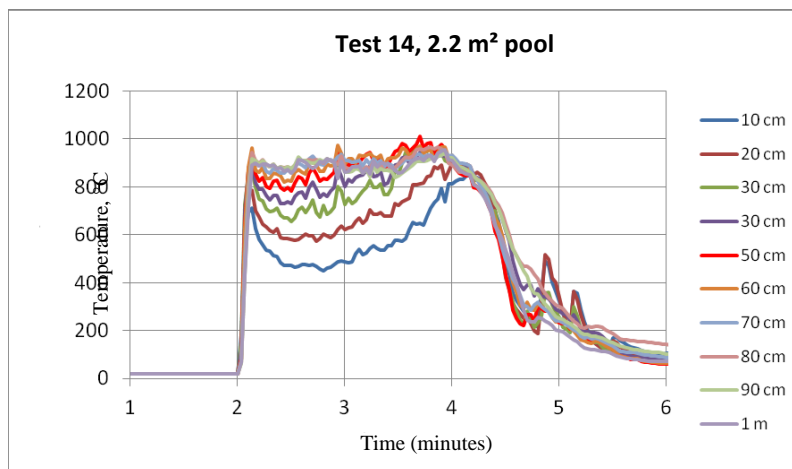
Figure 16. Temperature readings at different heights above a 2.2 m 2 pool fire
