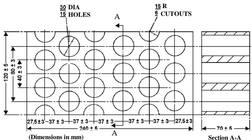
Figure 28 Dimension of Firebricks
