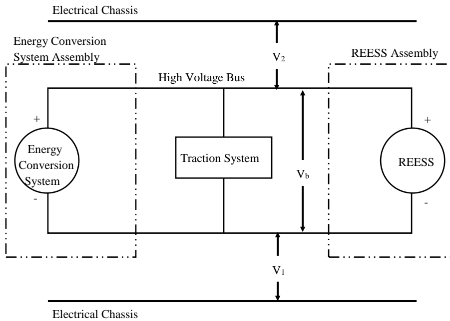
Figure 2 Measurement of V_b , V_1 , V_2
