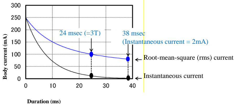
Figure 8 Body Current for 0.2 J and 200 V Capacitor under Large Area Hand-to-Hand Contact Under Wet Conditions (800 \Omega Body Resistance)
