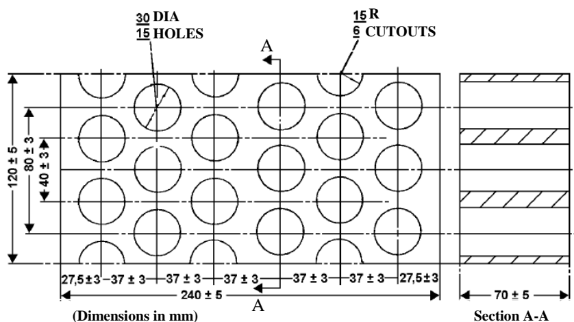
Figure 13 Dimension of Firebricks
