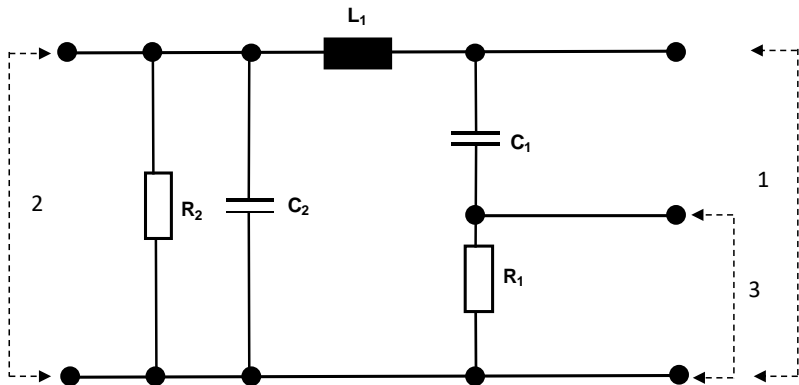
Figure 1 HV-AN artificial network
