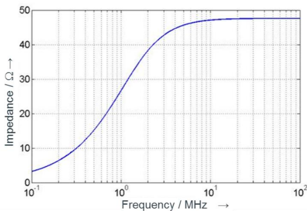
Figure 5 Impedance of DC-charging-AN
