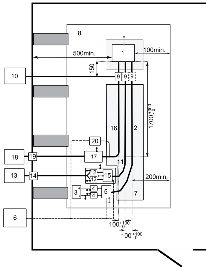
Top view (example of substitution method)
