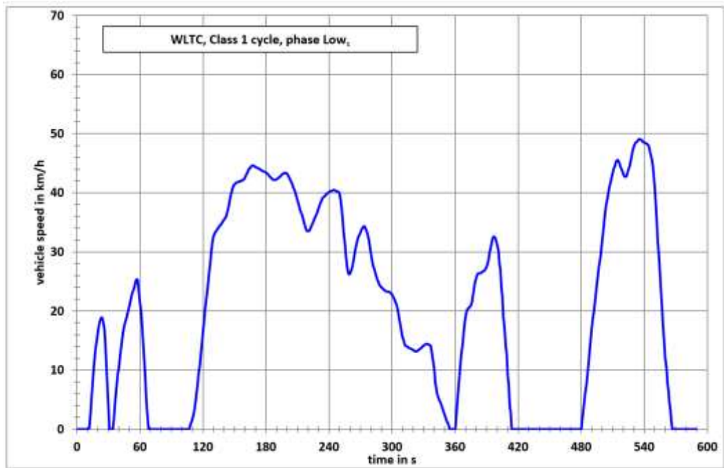
Figure A1/1 WLTC, Class 1 cycle, phase Low 1
