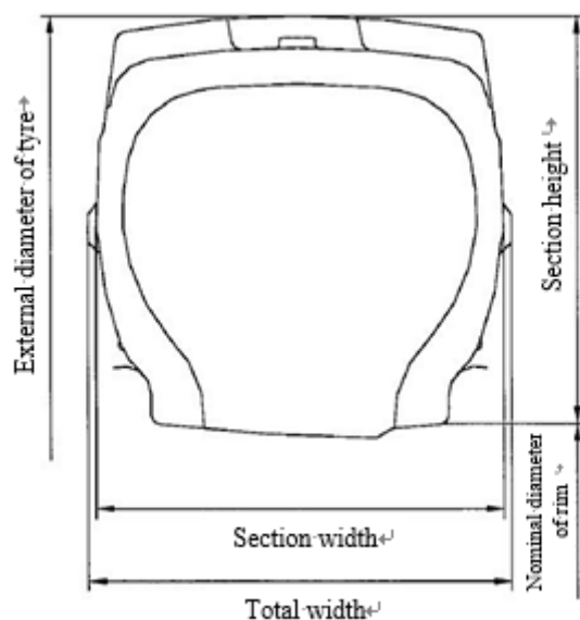
Figure x1 Schematic diagram of dimensional measurement of tire
