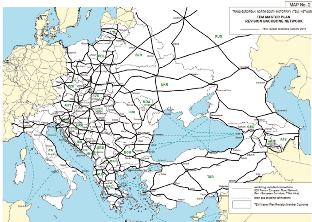
Figure 2.1 TEM Master plan revision backbone network
