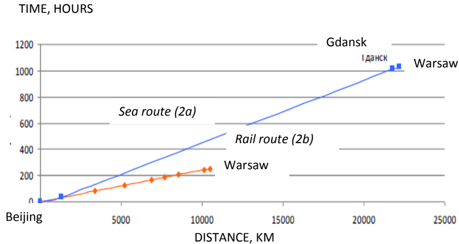
Figure 1.51 Time – distance diagram for routes 2a and 2b
