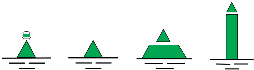
2.A Buoy with light 2.B Buoy without light 2.C Float with a topmark 2.D Spar (fig. 3.2)
