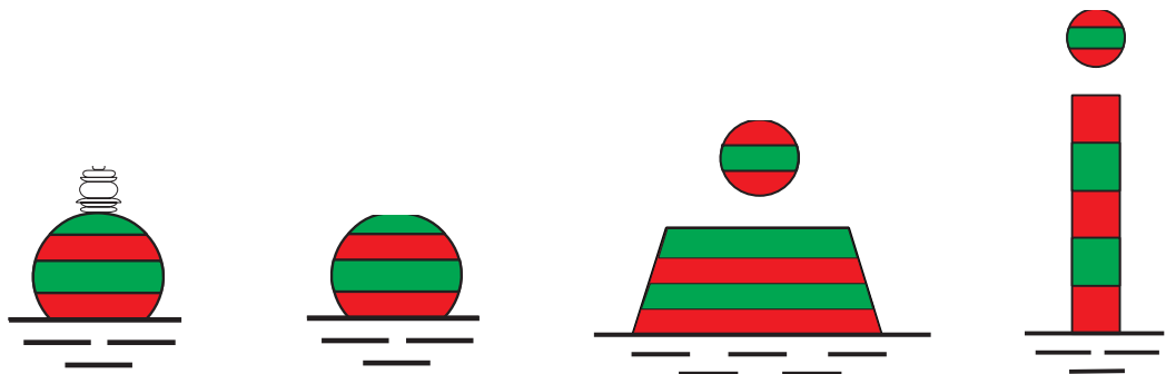
3.A Buoy with light 3.B Buoy without light 3.C Float with a topmark 3.D Spar (fig. 3.3)
