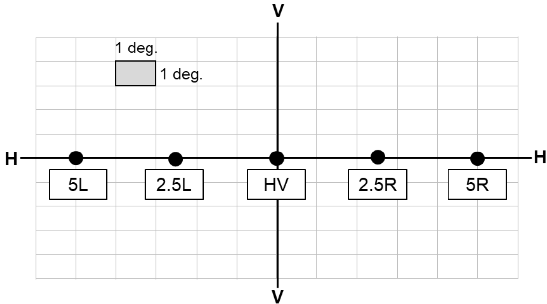
Figure A4-II Driving beam test points
