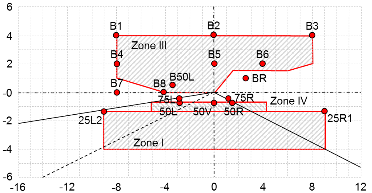
Figure A4-V Passing-beam for right-hand traffic
