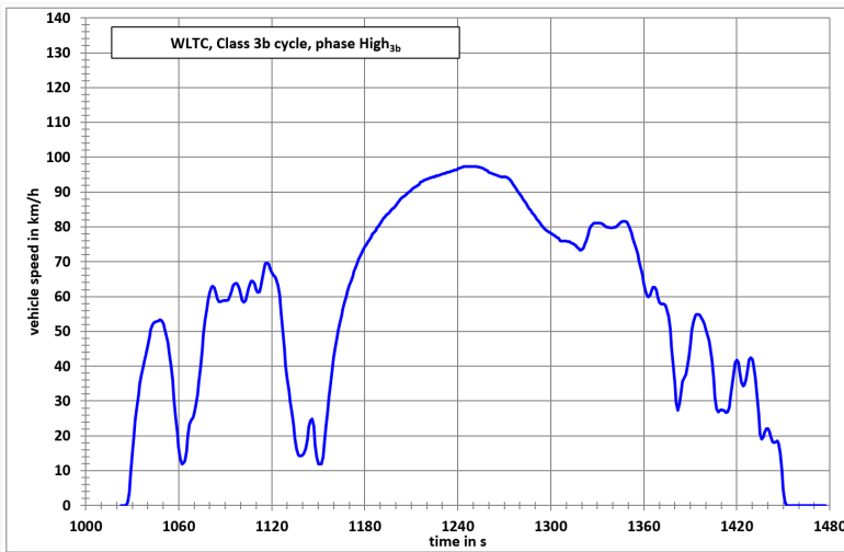
Figure A1/11 WLTC, Class 3b cycle, phase High 3b
