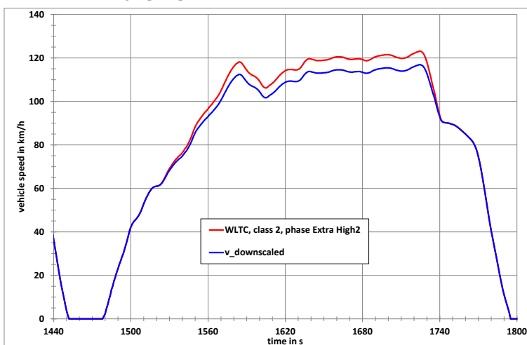
Figure A1/15 Downscaled extra high speed phase of the Class 2 WLTC
