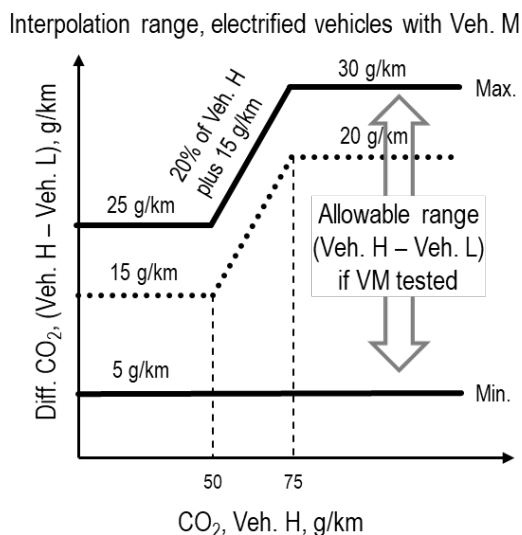
Figure A8/4 Interpolation range for EVs with vehicle M
