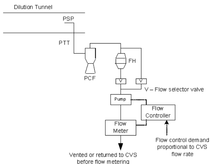
Figure A5/12 Particulate sampling system
