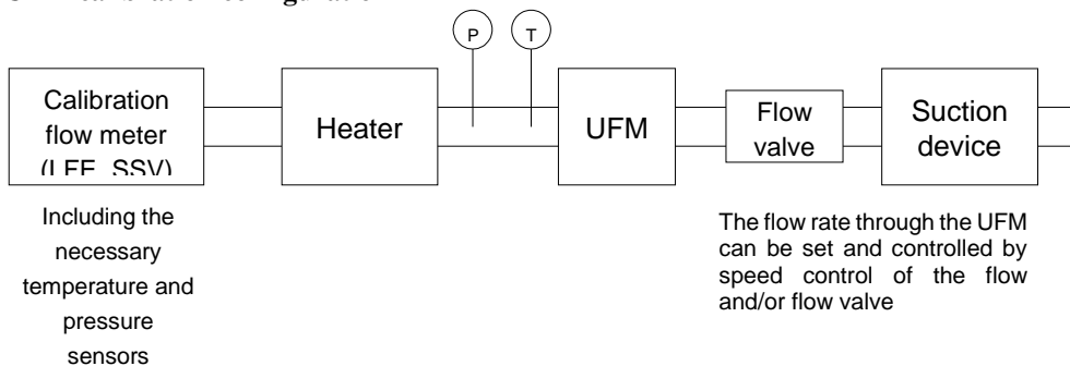
Figure A5/8 UFM calibration configuration
