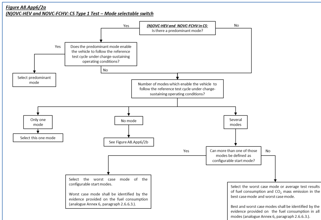
Figure A8.App6/2a and Figure A8.App6/2b Selection of a driver-selectable mode for OVC-HEVs, NOVC-HEVs and NOVC-FCHVs under charge-sustaining operating condition
