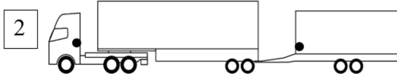
Figure 3 — tractor + A-semi + centre axle trailer
